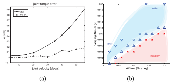
Fig. 2. Left picture: mean \bar{e} and standard deviation \sigma_e of the joint torque error from the elbow joint of iCub's right arm. Standard deviation is evidently bilinear with the increase of velocity, while the error mean is linearly proportional to the velocity. Polynomial fitting models are \sigma_e = 1.254\dot{q}^2 - 0.351\dot{q} + 0.057 and \bar{e} = 0.213\dot{q} - 0.049 respectively. Right picture: experimental evaluation of the stiffness-damping relationship. The lower region highlighted in red causes unstable behaviors of the arm when reaching its equilibrium point after an external force is applied. Boundary values were detected by overshoot of a step response. The light blue region shows feasible values, which make the joint behave like a softer or stiffer spring. The boundary region between the two can be ideally described by the following relationship: K_D = 0.075K_P - 0.0015 .
