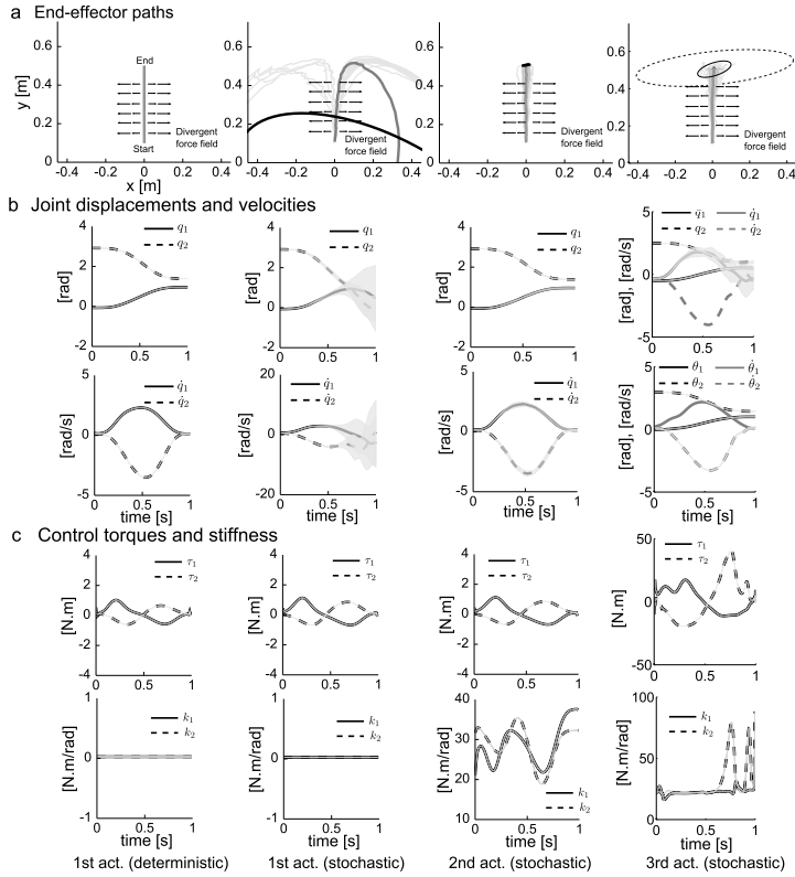
Fig. 1. A. Two-link arm moving in a divergent force field. The four columns depict the result obtained with the different type of actuators. a: End-effector trajectories. Light gray lines depict trials (20 are depicted). The thicker gray line is the mean path, and a shaded area depicts the standard deviation around the mean when possible. At the end, 95% confidence ellipses are displayed to show the variability of task accuracy. b: Joint displacements and velocities. Mean values and standard deviation (shaded areas) are plotted. c: Feedforward control commands for both the torque and stiffness. Note that, for all trials (i.e. noise instances) the same control is used (no use of feedback). For the 4th column, note the dashed-line ellipse shows the variability we obtain when the inertia matrix B is reduced by a factor 10. B. Single-joint arm subject to time delays. a: Angular displacements for 20 trials. 1st col.: feedforward control strategy without delays. 2nd col.: delayed feedback control strategy without stiffness. 3rd col.: Feedforward control strategy with 200 ms of delay, without using the optimal feedback gain L but using stiffness control. b: Angular velocities. c: Control trajectories.
