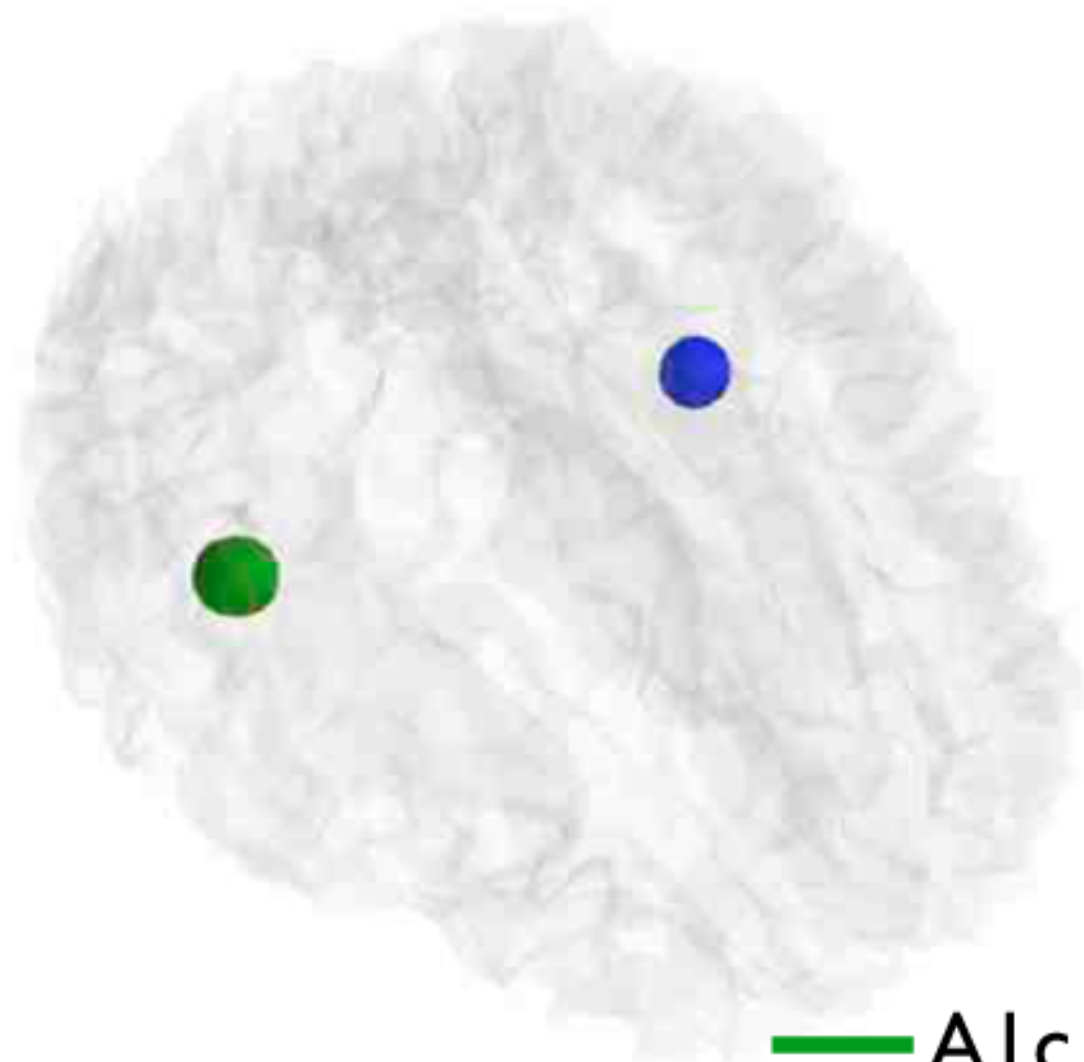
(b) \mathbf{GX}_{\text{TF-MxNE}}^* (explained data)
