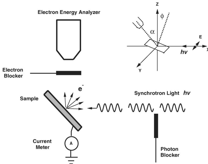
Fig. 1. Schematic of photoemission setup. A pulsed light is incident on the sample, kicking out electrons, and the electrons are collected by the electron energy analyzer. The photon blocker is used to change photon flux while keeping the beamline intact. The electron blocker is used to change the number of electrons collected by the analyzer. The sample current recorded by a picoammeter measures the number of electrons out of the sample which is proportional to the photon flux. In the upright, inset shows the measurement geometry of the light, the sample and the analyzer. The synchrotron light is along the X axis, with its electrical field E in the XY horizontal plane and parallel to Y axis. The sample normal is in the XZ plane and its angle with respect to the Z axis is referred to as \varphi . The analyzer is rotatable and the lens axis is in the YZ plane. The angle of the lens axis with respect to the Z axis is referred to as \alpha .
