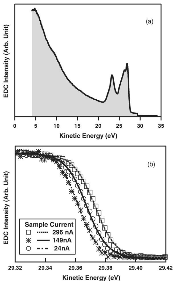
Fig. 2. Photoemission spectra of a polycrystalline gold measured at a photon energy of 34 eV and a temperature of 20 K. (a) Large energy range spectrum showing a Fermi cut-off at 29.38 eV, the valence band between 20 and 30 eV, and lower energy part arising from secondary electrons. (b) Au Fermi level measured at different photon flux, as indicated by different sample current. The open circles are experimental data which are fitted by Fermi–Dirac functions (lines).
