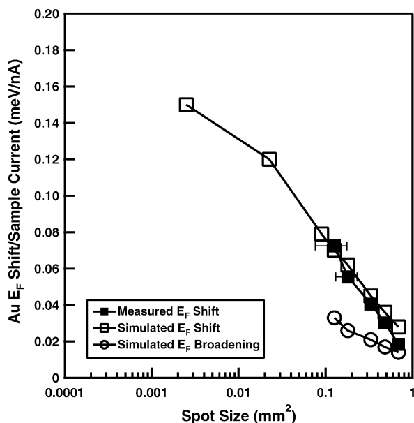
Fig. 6. Effect of beam spot size on the energy shift and broadening. The measured energy shift (solid square) is obtained from the slope by fitting the curves in Fig. 5a with linear lines. The simulated energy shift (open square) and broadening (open circle), are calculated by considering both the space and mirror charge effects and the overall gold valence band as shown in Fig. 2a.
