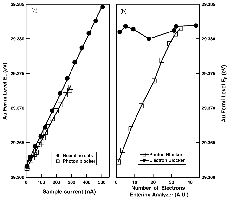
Fig. 3. Fermi level shift in photoemission process. The sample tilt angle \varphi is 45^\circ and the analyzer angle \alpha is 0. (a) Fermi level shift with the sample current varied by either varying the beamline slits (solid circle) or by using the photon blocker (open square). (b) Fermi edge shift as a function of the number of electrons entering the analyzer varied by either changing the photon flux by using the photon blocker (open square) or keeping the photon flux constant but using the electron blocker (solid circle).
