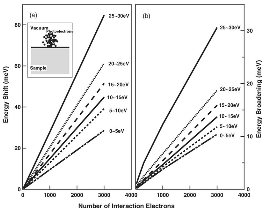
Fig. 10. Numerical calculations of space charge effect. The pulse length is 60 ps and the spot size is 0.43 \text{ mm} \times 0.42 \text{ mm} . (a) The energy shift as a function of the number of interaction electrons from the space charge effect. The test electron has an energy of 30 eV. Each curve represents the energy shift from the interaction electrons with an energy range of 0–5, 5–10, 10–15, 15–20, 20–25, and 25–30 eV. (b) The corresponding energy broadening from the space charge effect for those six different energy regions. The inset of (a) illustrates the space charge effect that shows a number of electrons (solid circles) in a pulse escaping from the sample surface.
