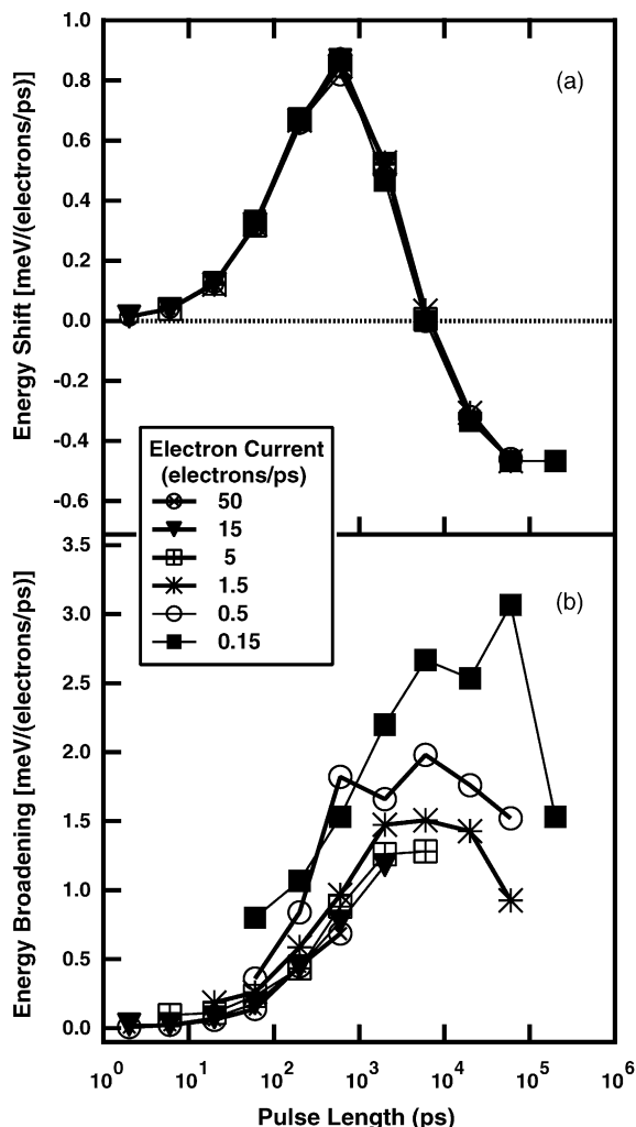
Fig. 14. (a) Energy shift and (b) broadening per electron current (the unit is electrons per picosecond (e/ps)) as a function of pulse length at different electron currents. The spot size is 0.43 \text{ mm} \times 0.42 \text{ mm} . For the energy shift, all curves overlap with each other, indicating that the energy shift is proportional to the electron current. But for the energy broadening, they do not strictly overlap with each other, particularly at longer pulse length.
