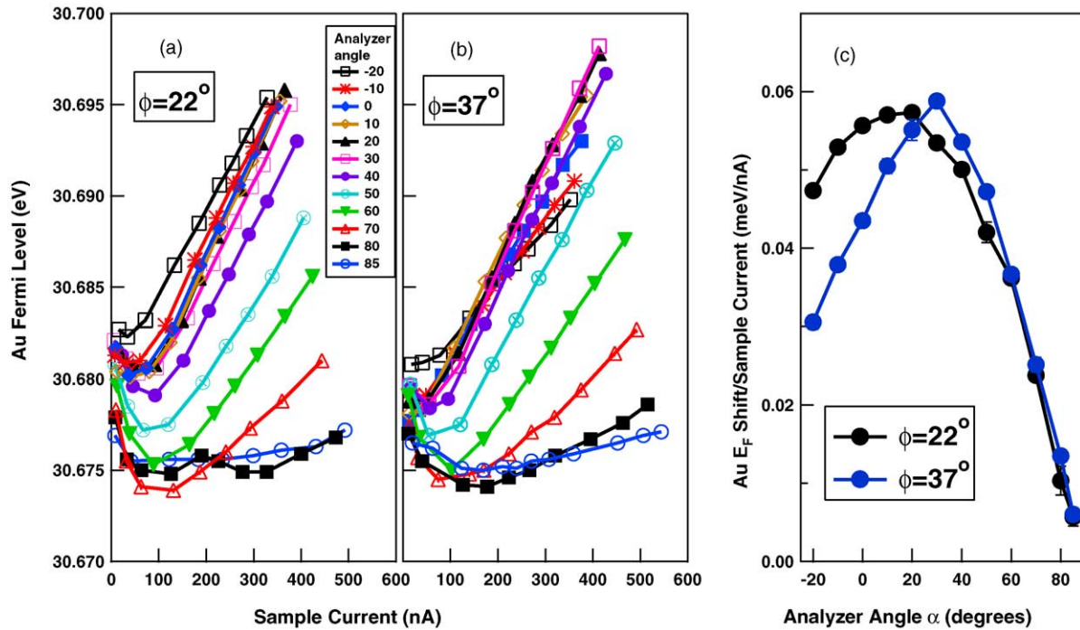
Fig. 8. Energy shift as a function of sample current at different analyzer angles for the sample tilt angle of (a) \phi = 22^\circ and (b) \phi = 37^\circ . The spot size for these two cases is approximately 0.4\text{ mm} \times 0.4\text{ mm} . Note that while for the small analyzer angle the energy shift changes nearly linearly over the entire sample current range, for large analyzer angle, it shows a back bend at low sample current. If we take the value near zero sample current as the intrinsic Fermi level, it is found that the energy shift at high analyzer angle can be negative. (c) Energy shift per sample current for two different sample tilt angles. The slope is obtained by fitting the straight high sample current part as in Fig. 8.
