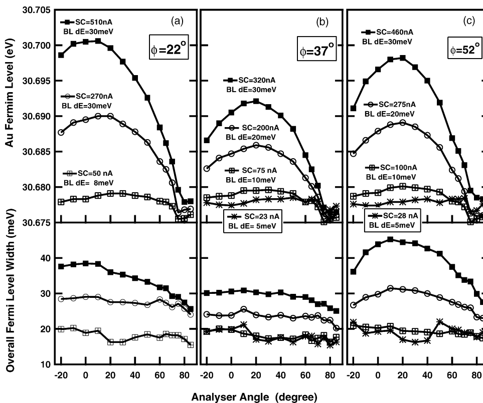
Fig. 7. The energy shift (upper panel) and broadening (lower panel) as a function of the analyzer angle \alpha for different sample tilt angles (a) \varphi = 22^\circ , (b) \varphi = 37^\circ , and (c) \varphi = 52^\circ . The curves in each panel represent different sample currents (SC) under a given beamline resolution ( dE ). For any given curve the sample current is nearly a constant.
