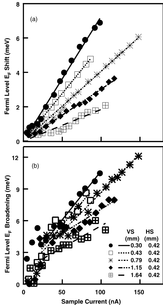
Fig. 5. (a) Effect of beam spot size on the energy shift. The energy shift for each spot size (FWHM) shows a nearly linear dependence on the sample current and is fitted with a straight line (solid lines). The sample tilt angle \varphi is 45^\circ and the analyzer angle \alpha is 0. (b) Effect of beam size on the energy broadening. The broadening at high sample current can be approximated as a straight line; the solid lines also act as a guide to the eye.
