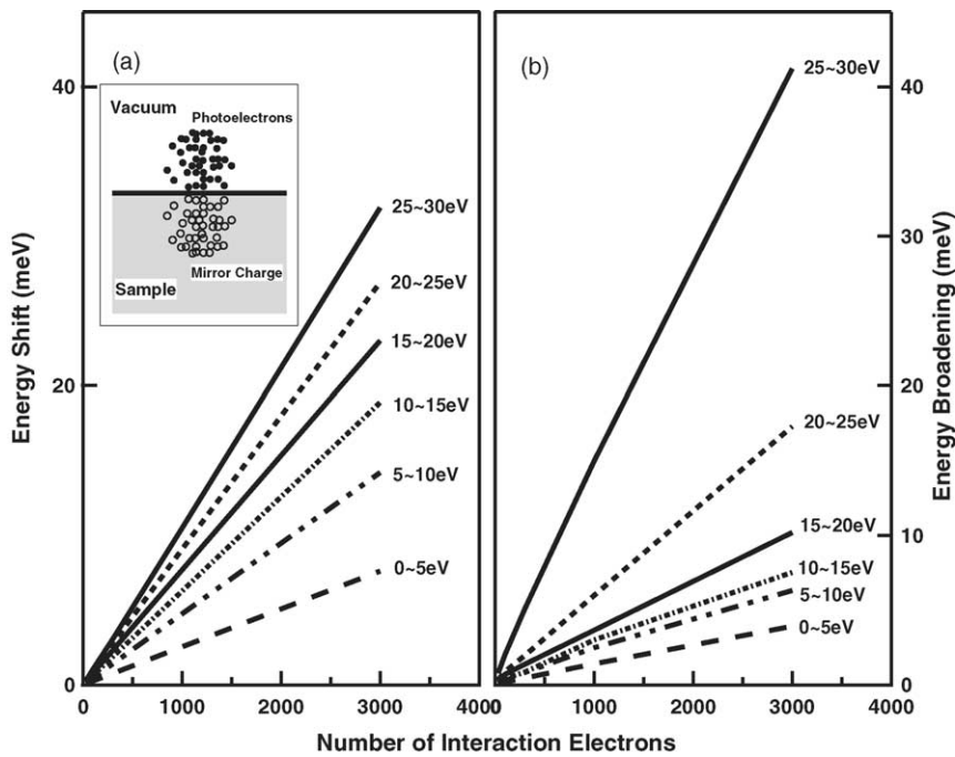
Fig. 12. Numerical calculations of combined space and mirror charge effect. The pulse length is 60 ps and the spot size is 0.43 mm × 0.42 mm. (a) The energy shift as a function of the number of the interaction electrons from both space charge and mirror charge effects. The test electron has an energy of 30 eV. Each curve represents the energy shift from the interaction electrons with an energy range of 0–5, 5–10, 10–15, 15–20, 20–25, and 25–30 eV. (b) The corresponding energy broadening from both space charge and mirror charge for those six different energy regions. The inset of (a) schematically shows the mirror charge effect: a pulse of electrons (solid circles) escaping from the sample surface and each electron has a mirror charge (open circles) inside the sample.
