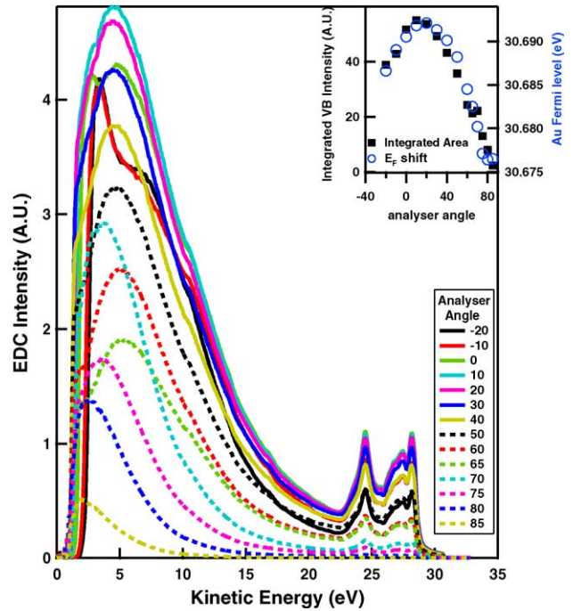
Fig. 9. Large energy-range valence band of Au measured at different analyzer angle \alpha . The sample tilt angle is \phi = 37^\circ . In the inset shows the integrated spectral weight over the entire energy range of 5–35 eV as a function of the analyzer angle \alpha (black solid square). For comparison, the Fermi level as a function of the analyzer angle measured under similar condition is also plotted (blue circle).
