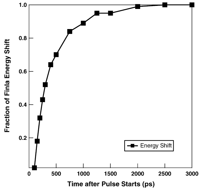
Fig. 13. Time evolution of the energy shift. The data are obtained by averaging for 9, 30, 90, and 300 electrons/pulse.
