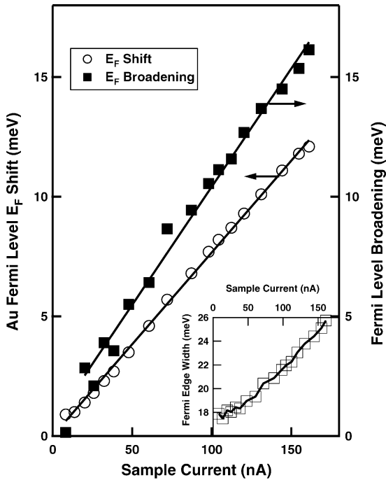
Fig. 4. Fermi edge broadening (solid square) and the Fermi edge shift (open circle) as a function of sample current. The sample tilt angle \varphi is 45^\circ and the analyzer angle \alpha is 0. The beam spot size is \sim 0.43 \text{ mm} \times 0.30 \text{ mm} . The photon flux corresponding to 150 nA sample current is \sim 5 \times 10^{13} photons/second. The inset shows the measured overall Fermi edge width as a function of the sample current, which includes all contributions including the beamline, the analyzer and the temperature broadening. The net broadening resulting from pulsed photons is obtained by deconvolution of the measured data, taking the width at low photon flux as from all the other contributions.
