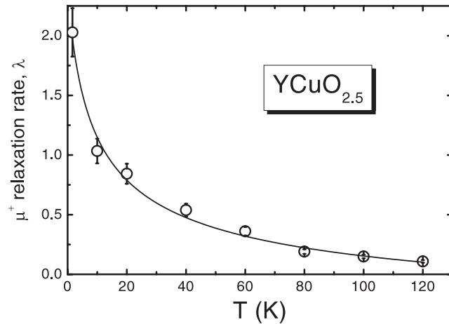
Figure 2. Muon relaxation rate, \lambda , versus T in \text{YCuO}_{2.5} . \lambda is extracted from a square root fit of the asymmetry A(t) = A(0) \exp(-\sqrt{\lambda t}) under H_{\text{LF}} = 20 G versus time. Notice the progressive increase without any sharp feature, which also supports the absence of any phase transition.
