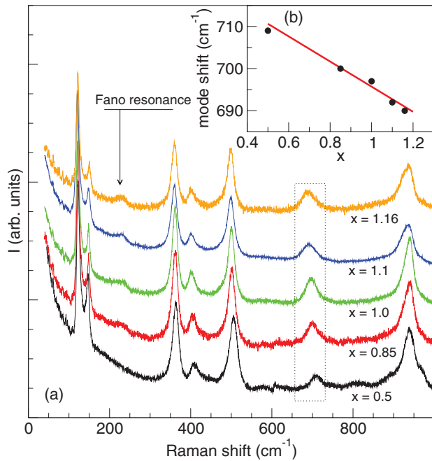
FIG. 6. (Color online) (a) Raman spectra for \text{Zn}_x\text{Cu}_{4-x}(\text{OH})_6\text{Cl}_2 with x = 0.5, 0.85, 1.0, 1.1, and 1.16 . The spectra are shifted in intensity for clarity. (b) The linear frequency dependence of the phonon mode at 700 \text{ cm}^{-1} [indicated by the box in panel (a)], with the Cu/Zn ratio.
