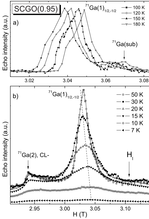
FIG. 8: ^{71}\text{Ga} spectra in SCGO ( H_l = 2\pi\nu_l/^{71}\gamma ). a) High temperature. The ^{71}\text{Ga}(2) contribution appears as a flat background in this field range. b) Low temperature, lines are broadened. The ^{71}\text{Ga}(2) contribution remains flat at the position of the ^{71}\text{Ga}(1) line, which shifts to higher fields in this temperature region when the temperature decreases.
