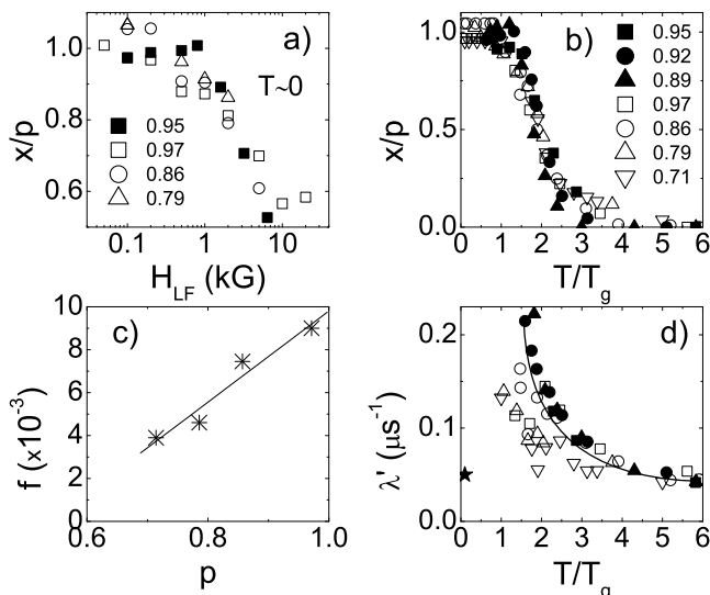
FIG. 24: Fitting parameters of Eq. 6 for BSZCGO and SCGO (open and full symbols). f is common for both systems.
