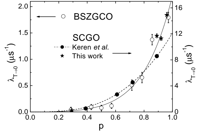
FIG. 22: p -dependence of \lambda_{T \rightarrow 0} for BSZCGO( p ) (open symbols) and SCGO( p ) (full symbols). Continuous (dashed) lines are \sim p^3 + 1.9(3)p^6 ( \propto p^3 , [57]) fits.
