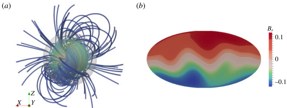
FIGURE 6. (Colour online) (a) Streamlines of \mathbf{B}_T extended to one radius outside the sphere. (b) The Mollweide projection of the radial component B_r of \mathbf{B}_T at the surface of the sphere. The vector field \mathbf{B}_T has been rotated such that the dominant dipole axis is vertical.
